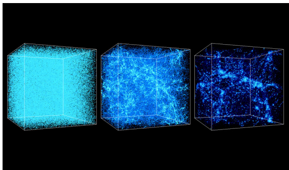
Simulation of the formation of clusters and large-scale filaments in the CDM model with dark energy, from z \approx 30 (l), to z \approx 5 (m), to present (r); box dimension = 43 million parsecs. (A. Kravtsov and A. Klypin)
