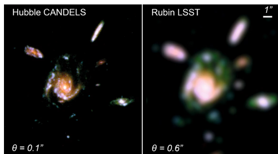
Comparison of Hubble and expected Rubin Observatory LSST data resolution. (L) BVz color image from the Hubble CANDELS field with \theta = 0.1'' and r \approx 28.5 . Roman will have comparable resolution. (R) Simulated Rubin LSST image made by degrading Hubble data to Rubin resolution of \theta = 0.6'' . In the Rubin image, the galaxy is blended with surrounding objects. Correlating overlapping Rubin and Roman imagery would make it possible to develop machine learning algorithms to deblend Rubin imagery that does not overlap with Roman. (B.E. Robertson, et al. 2019, Nat Rev Phys, 1, 450)
