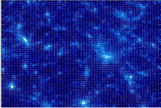
Simulation of cosmic shear in a CDM model. Line segments represent amplitude and direction of lensing shear produced by over-densities (light blue) and voids (dark blue). (B. Jain, U. Seljak, & S. White 2000, ApJ, 530, 547)
