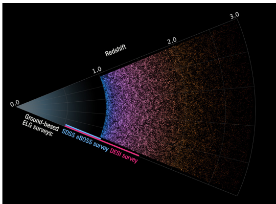
Visualization of simulated Roman emission-line galaxy distribution data used to measure BAO and RSD. The wedge shown covers an RA sweep of 45^\circ with a DEC thickness of 1^\circ , and includes more than 215,000 galaxies. (Data provided by Z. Zhai and Y. Wang, Caltech/IPAC. Visualization by J. DePasquale, STScI.)
